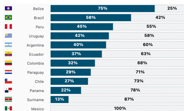
FMM: Undisbursed Amount (%), Disbursed Amount (%), by Country (only INV)
